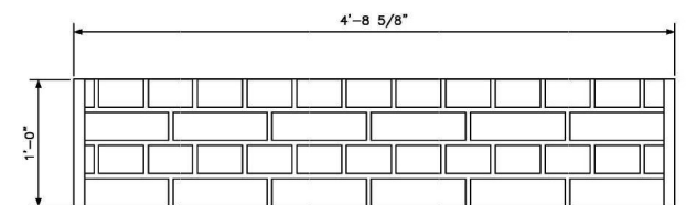
DETAILS - OLDBRICK WALL PANEL & CAP
