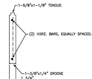
WALL PANEL - SECTION
