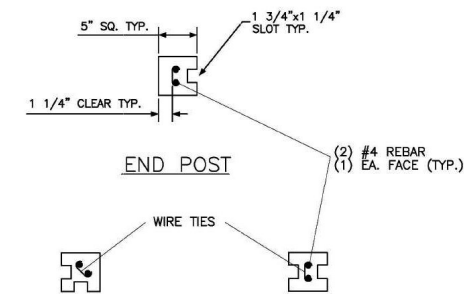
SECTION - 6' SCREENING WALL POST
