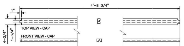
WALL PANEL CAP - PLAN VIEW & ELEVATION
