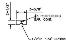
WALL PANEL CAP - SECTION
